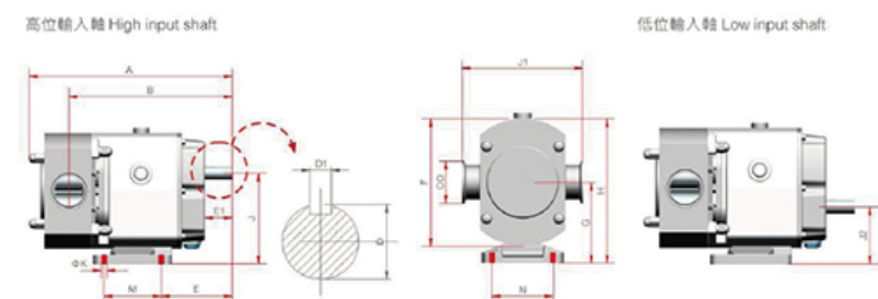
低位輸入軸 Low input shaft
